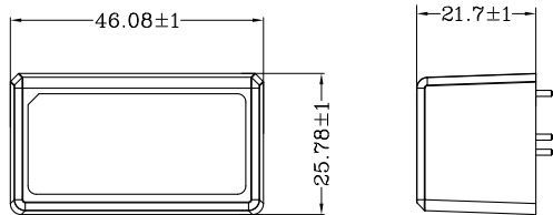
Dimensions:(mm)
