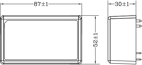
Dimensions:(mm)
