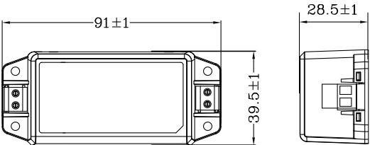
Dimensions:(mm)
