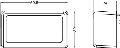
Dimensions:(mm)
