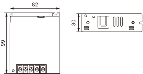
Dimensions:(mm)
