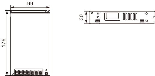
Dimensions:(mm)
