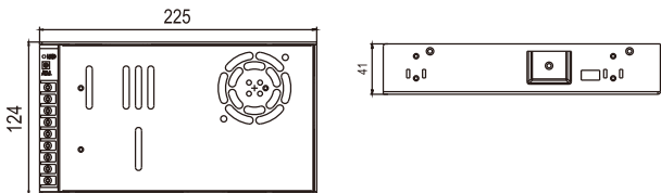
Dimensions:(mm)
